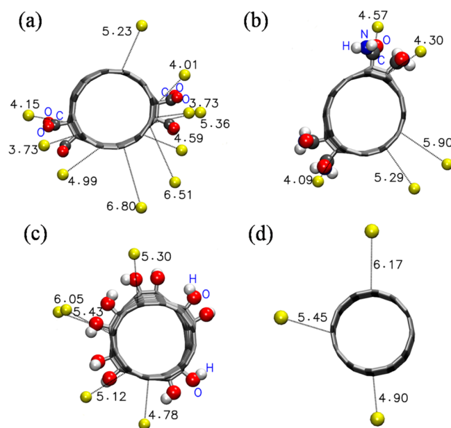
Figure 7. Snapshots of lead ( \text{Pb}^{2+} ) ion with functionalized CNT and bare CNT at 0.5 M concentration with in a 10 Å cutoff from the center line of CNT (a) \text{CNT}-\text{COO}^- , (b) \text{CNT}-\text{CONH}_2 , (c) \text{CNT}-\text{OH} , and (d) bare CNT.
