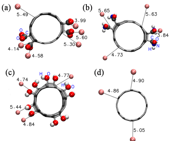
Figure 3. Snapshots of cadmium ( \text{Cd}^{2+} ) ion with functionalized CNT and bare CNT at 0.5 M concentration within a cutoff distance, 10 Å, from the center line of CNT (a) CNT- \text{COO}^- , (b) CNT- \text{CONH}_2 , (c) CNT- \text{OH} , and (d) bare CNT.
