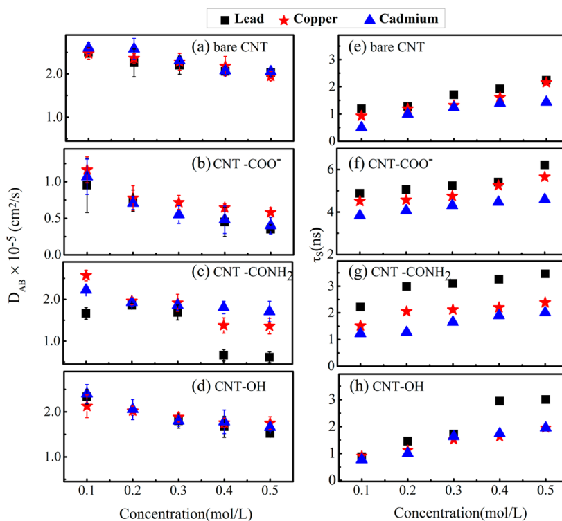
Figure 9. Effect of functional groups on the diffusion coefficient and residence time of metal ions at different concentrations of (a, e) bare CNT, (b, f) CNT-COO - , (c, g) CNT-CONH 2 , (d, h) CNT-OH.
