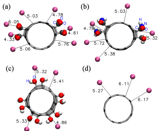
Figure 5. Snapshots of copper ( \text{Cu}^{2+} ) ion with functionalized CNT and bare CNT at 0.5 M concentration with a cutoff 10 Å from the center line of CNT (a) CNT- \text{COO}^- , (b) CNT- \text{CONH}_2 , (c) CNT- \text{OH} , and (d) bare CNT.
