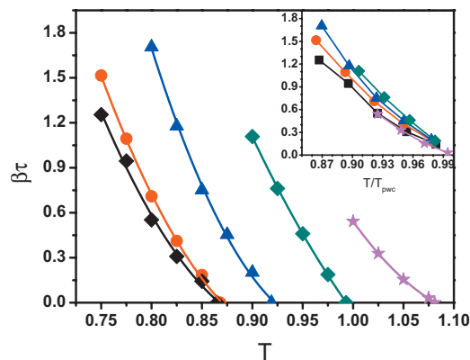
FIG. 12. Infinite system size boundary tension vs temperature for various association strengths. Curves serve as a guide to the eye. The inset represents the infinite system size boundary tension vs reduced temperature for different associating strengths. Symbols square, circle, triangle, diamond and star represent boundary tension for associating strength \varepsilon_{af}=2, 4, 6, 8, 10 , respectively.
